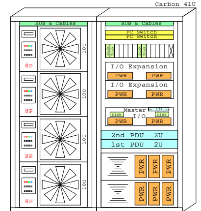
AS GS1280 M32 In 41U Cabinet
