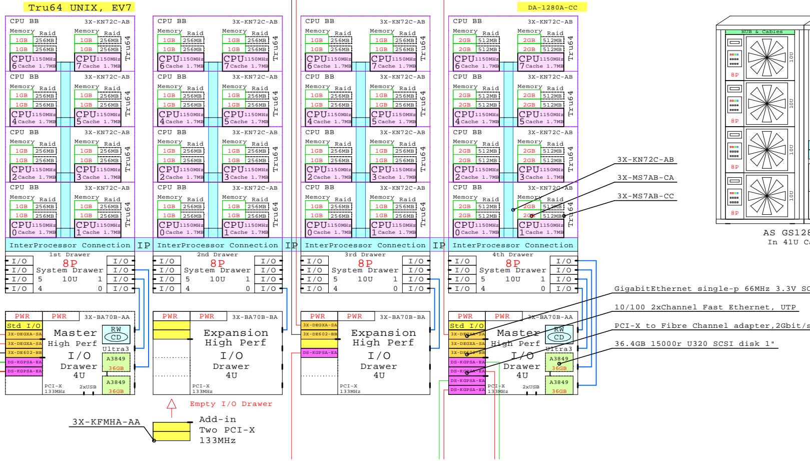
BOM for the first Master I/O Drawer, Left
